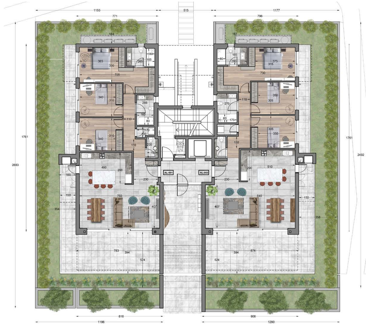
GROUND FLOOR
